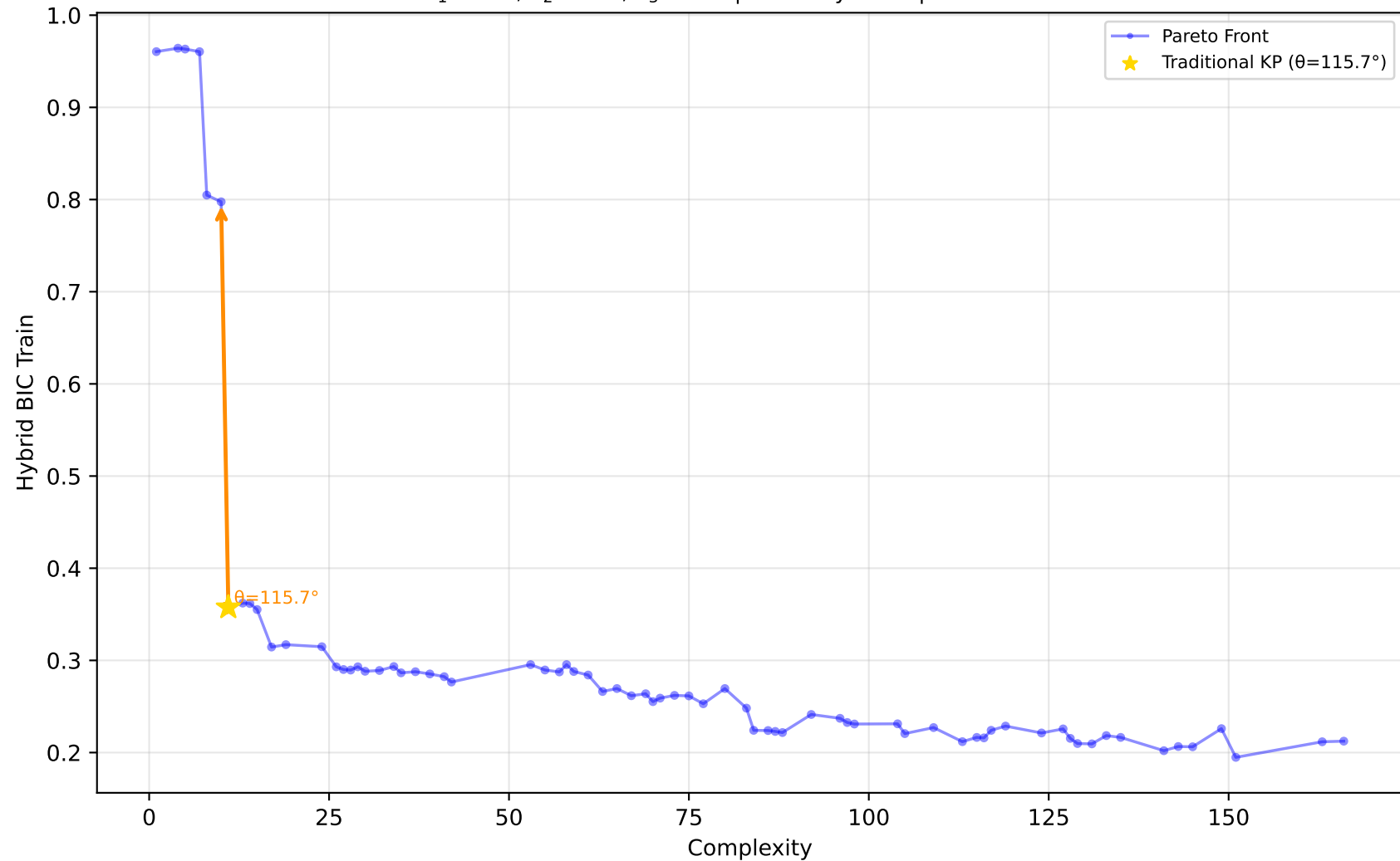
556_analcatdata_apnea2 - Run 9 - MVP - Hybrid BIC Train \lambda_1=0.00, \lambda_2=0.00, \lambda_3=0.00 | Difficulty: 0.82 | Method: hmr
