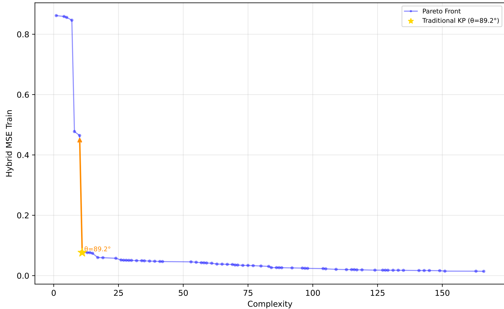
556_analcatdata_apnea2 - Run 9 - MVP - Hybrid MSE Train \lambda_1=0.00, \lambda_2=0.00, \lambda_3=0.00 | Difficulty: 0.82 | Method: hmr
