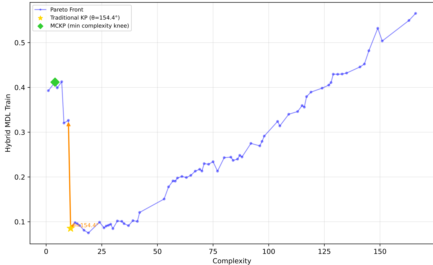
556_analcatdata_apnea2 - Run 9 - SVP - Hybrid MDL Train \lambda_1=0.00, \lambda_2=0.00, \lambda_3=0.00 | Difficulty: 0.82 | Method: hmr
