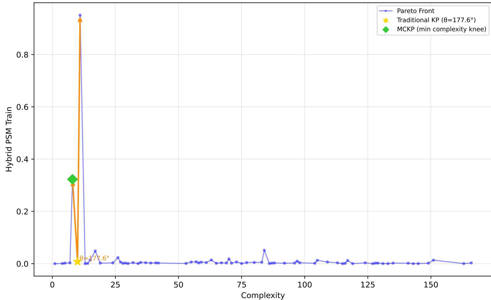
556_analcatdata_apnea2 - Run 9 - SVP - Hybrid PSM Train \lambda_1=0.00, \lambda_2=0.00, \lambda_3=0.00 | Difficulty: 0.82 | Method: hmr
