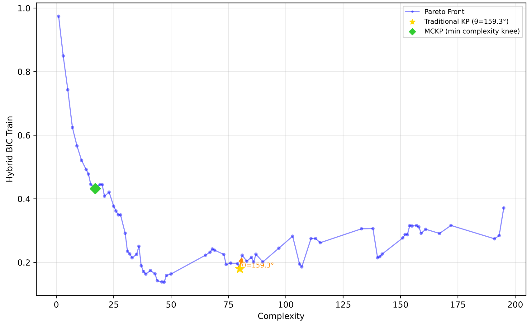
229_pwLinear - Run 10 - SVP - Hybrid BIC Train \lambda_1=0.50, \lambda_2=0.00, \lambda_3=0.00 | Difficulty: 1.00 | Method: hmr
