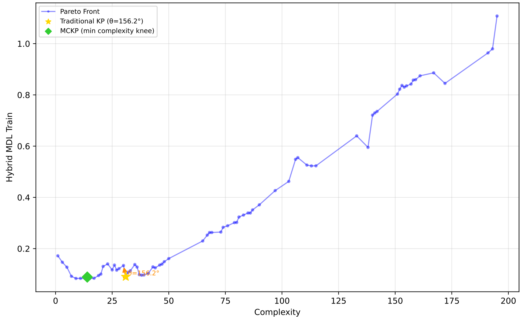
229_pwLinear - Run 10 - SVP - Hybrid MDL Train \lambda_1=0.50, \lambda_2=0.10, \lambda_3=0.00 | Difficulty: 1.00 | Method: hmr
