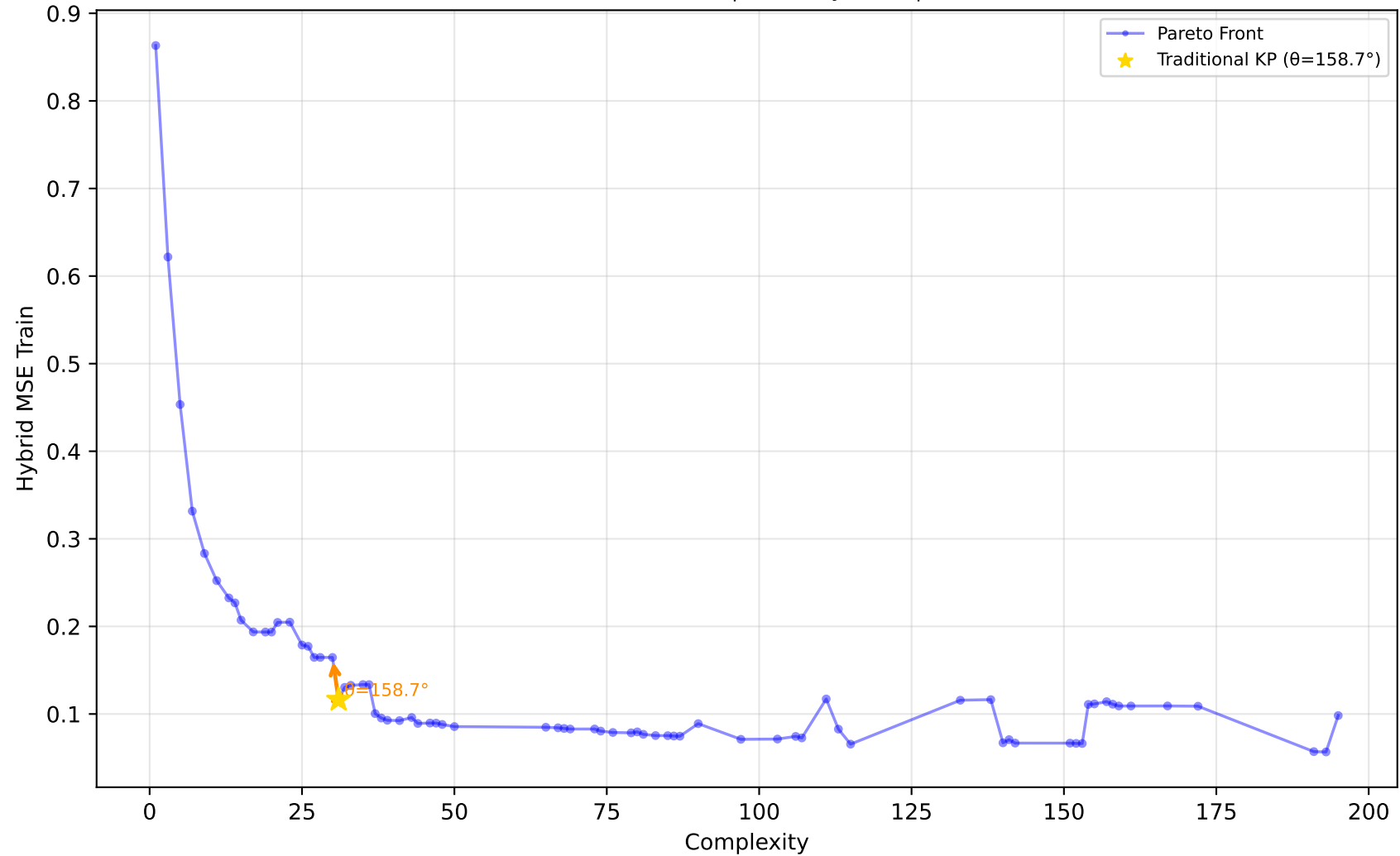
229_pwLinear - Run 10 - SVP - Hybrid MSE Train \lambda_1=0.50, \lambda_2=0.00, \lambda_3=0.00 | Difficulty: 1.00 | Method: hmr
