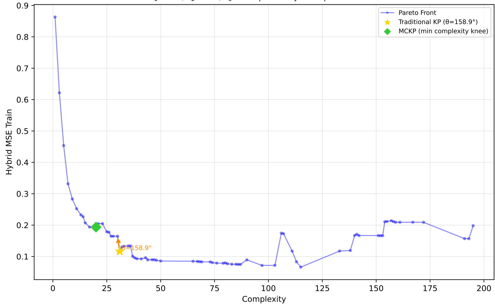
229_pwLinear - Run 10 - SVP - Hybrid MSE Train \lambda_1=0.50, \lambda_2=0.10, \lambda_3=0.00 | Difficulty: 1.00 | Method: hmr
