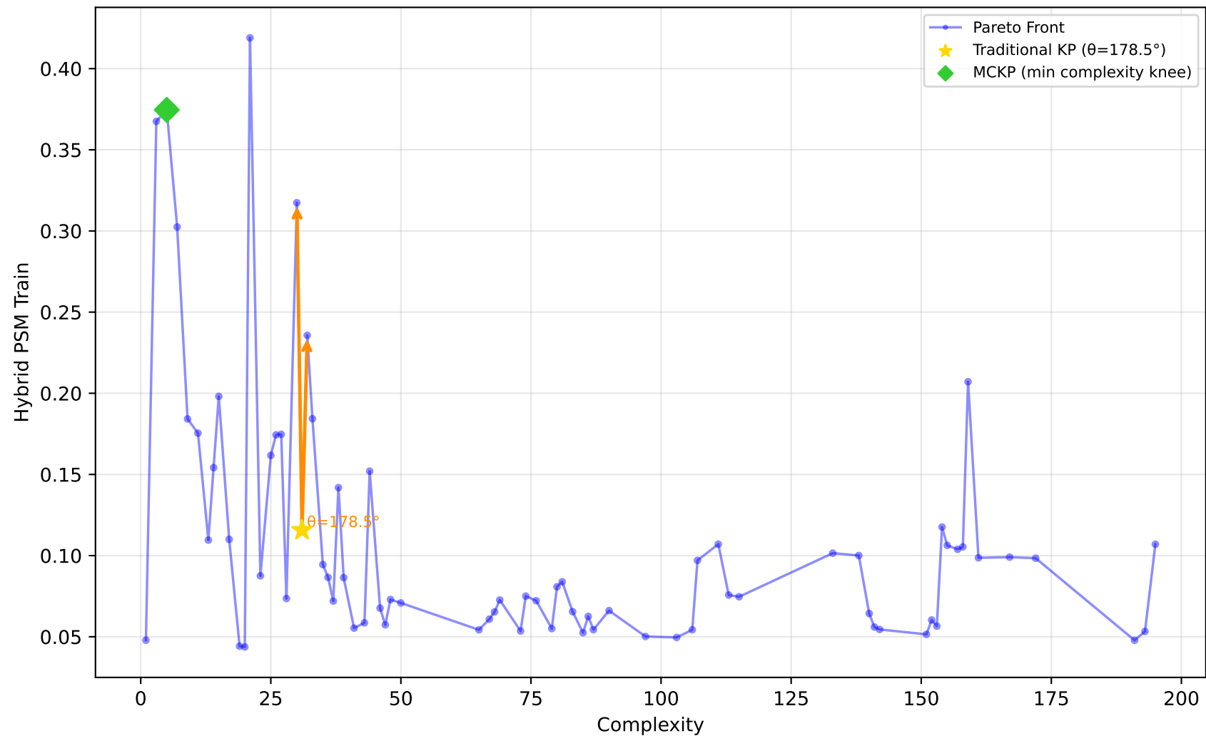
229_pwLinear - Run 10 - SVP - Hybrid PSM Train \lambda_1=0.50, \bar{\lambda}_2=0.00, \lambda_3=0.00 | Difficulty: 1.00 | Method: hmr
