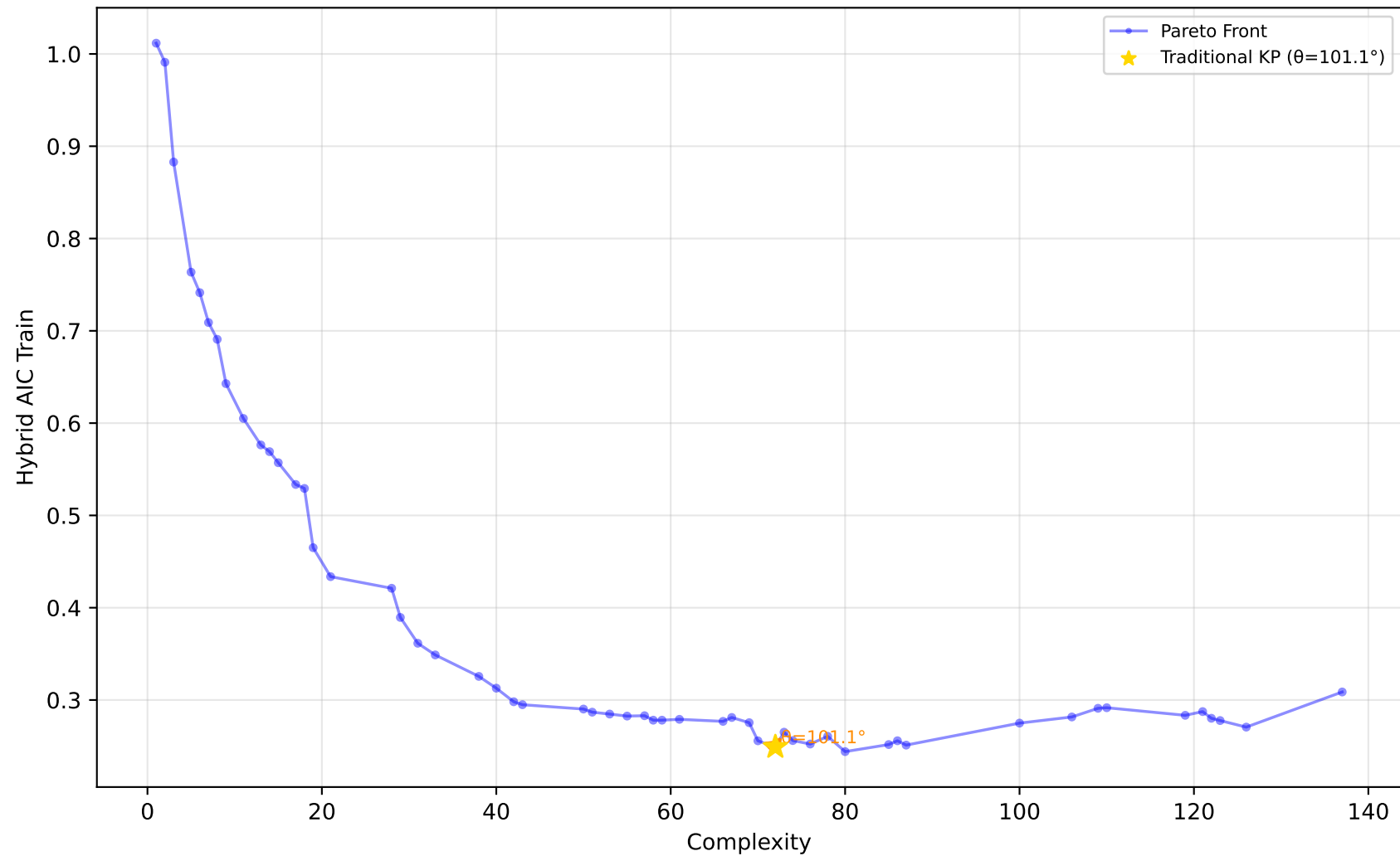
229_pwLinear - Run 11 - MVP - Hybrid AIC Train \lambda_1=0.50, \lambda_2=0.00, \lambda_3=0.00 | Difficulty: 1.00 | Method: hmr
