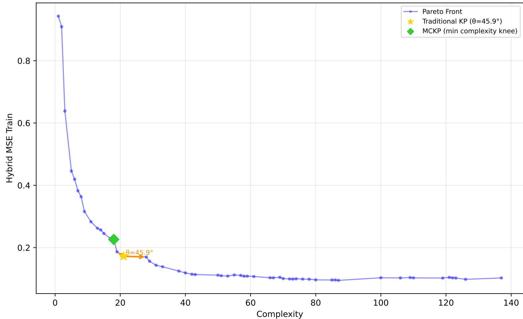
229_pwLinear - Run 11 - MVP - Hybrid MSE Train \lambda_1=0.50, \lambda_2=0.00, \lambda_3=0.00 | Difficulty: 1.00 | Method: hmr
