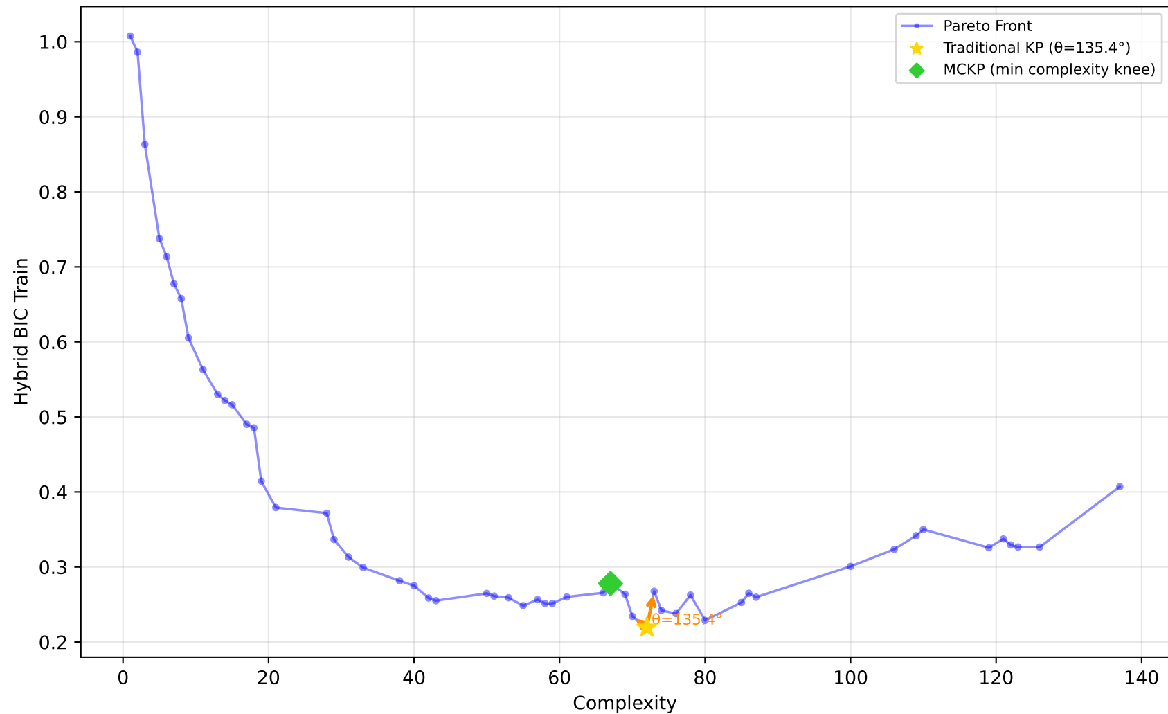
229_pwLinear - Run 11 - SVP - Hybrid BIC Train \lambda_1=0.50, \lambda_2=0.00, \lambda_3=0.00 | Difficulty: 1.00 | Method: hmr
