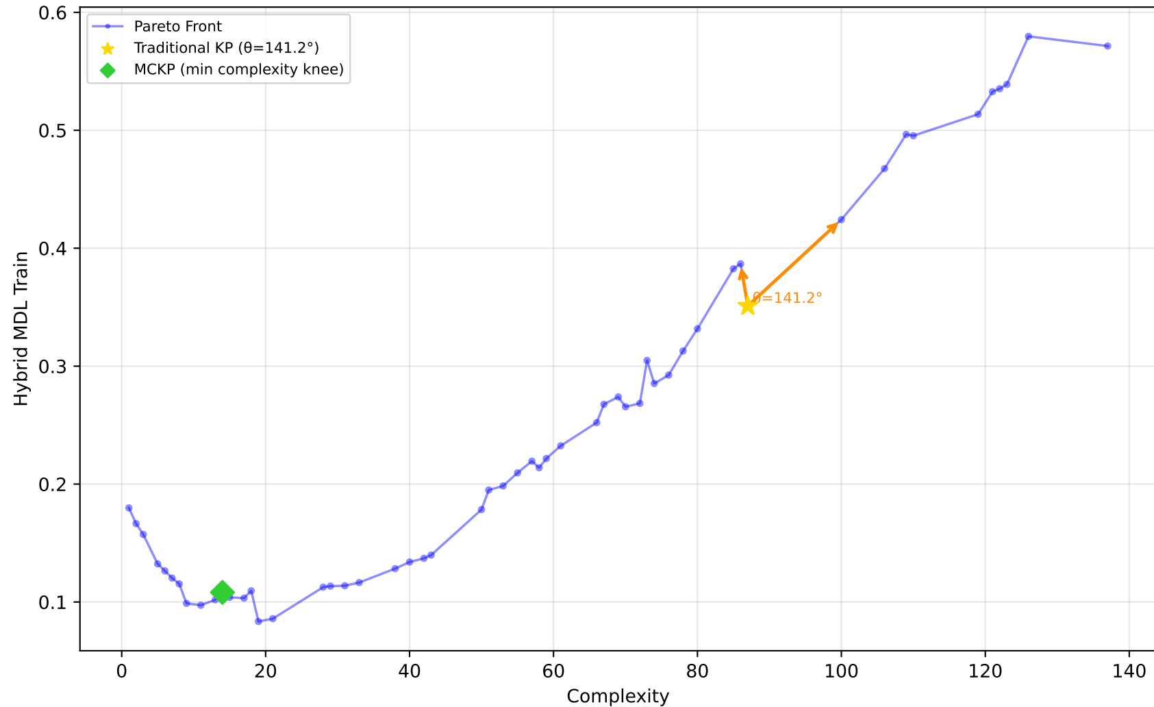
229_pwLinear - Run 11 - SVP - Hybrid MDL Train \lambda_1=0.50, \bar{\lambda}_2=0.00, \lambda_3=0.00 | Difficulty: 1.00 | Method: hmr
