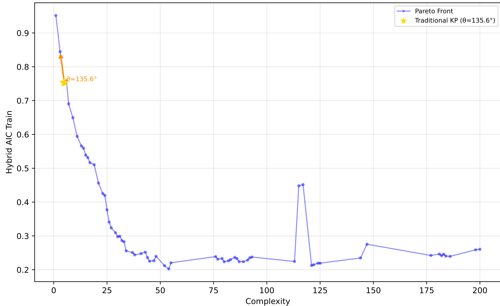
229_pwLinear - Run 12 - MVP - Hybrid AIC Train \lambda_1=0.50, \lambda_2=0.00, \lambda_3=0.00 | Difficulty: 1.00 | Method: hmr
