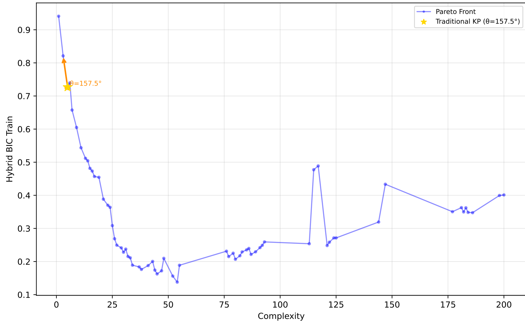
229_pwLinear - Run 12 - SVP - Hybrid BIC Train \lambda_1=0.50, \lambda_2=0.00, \lambda_3=0.00 | Difficulty: 1.00 | Method: hmr
