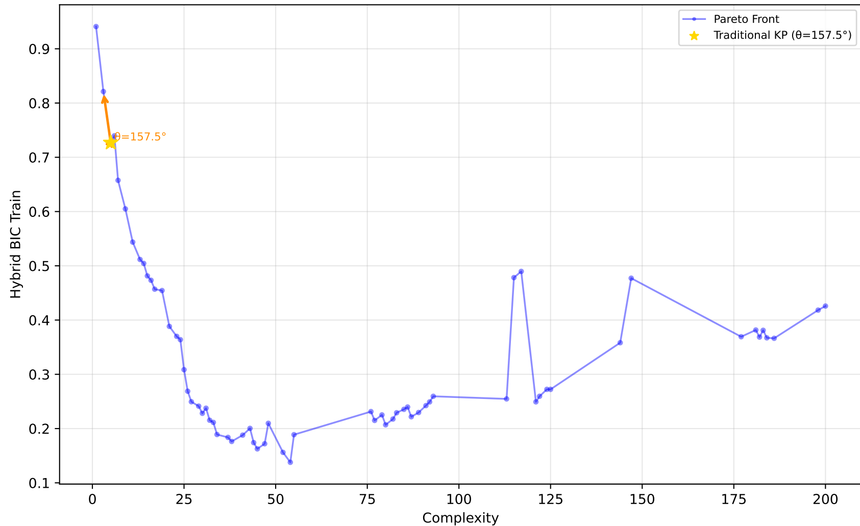
229_pwLinear - Run 12 - SVP - Hybrid BIC Train \lambda_1=0.50, \lambda_2=0.10, \lambda_3=0.00 | Difficulty: 1.00 | Method: hmr
