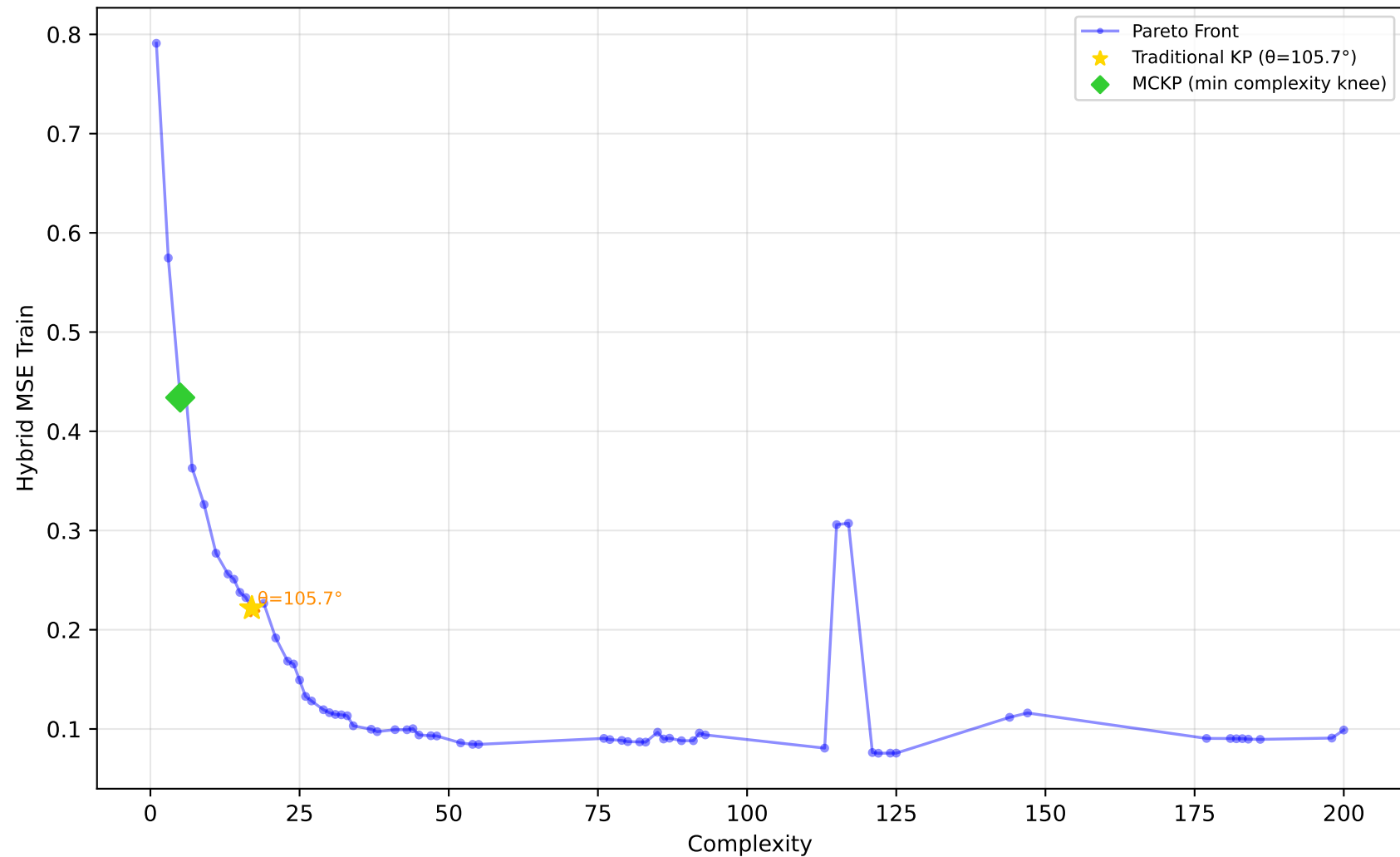
229_pwLinear - Run 12 - SVP - Hybrid MSE Train \lambda_1=0.50, \lambda_2=0.10, \lambda_3=0.00 | Difficulty: 1.00 | Method: hmr
