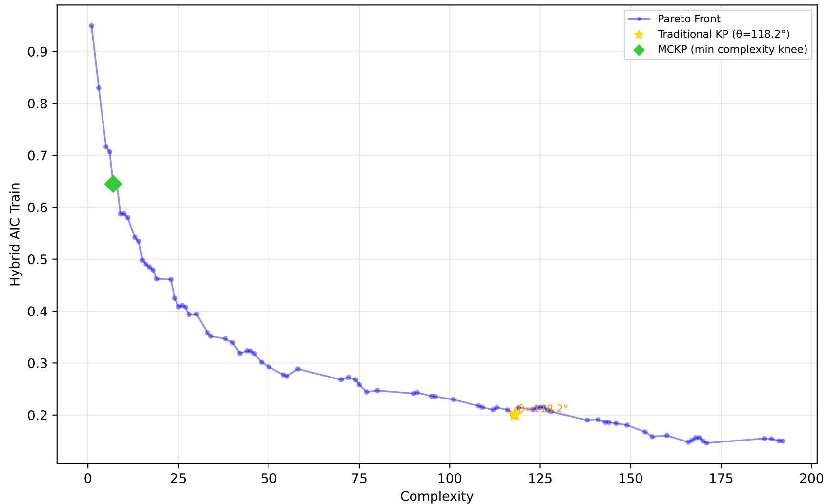
229_pwLinear - Run 13 - MVP - Hybrid AIC Train \lambda_1=0.50, \bar{\lambda}_2=0.00, \lambda_3=0.00 | Difficulty: 1.00 | Method: hmr
