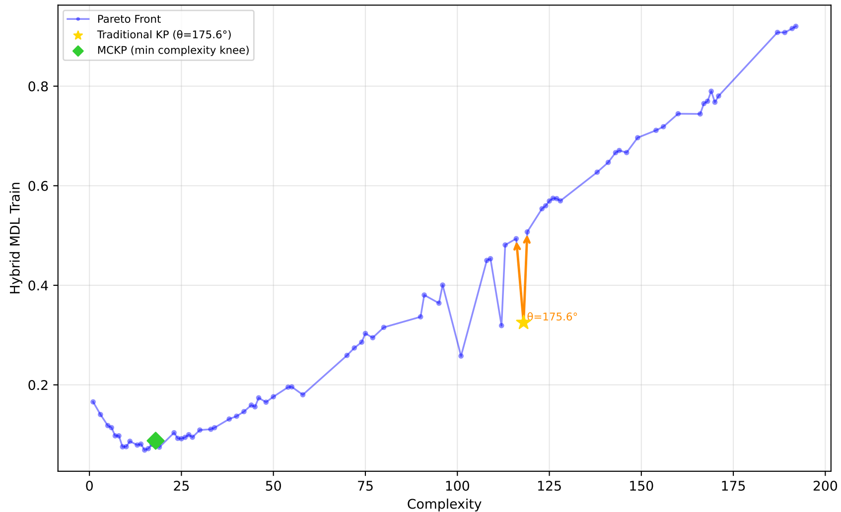
229_pwLinear - Run 13 - MVP - Hybrid MDL Train \lambda_1=0.50, \lambda_2=0.00, \lambda_3=0.00 | Difficulty: 1.00 | Method: hmr
