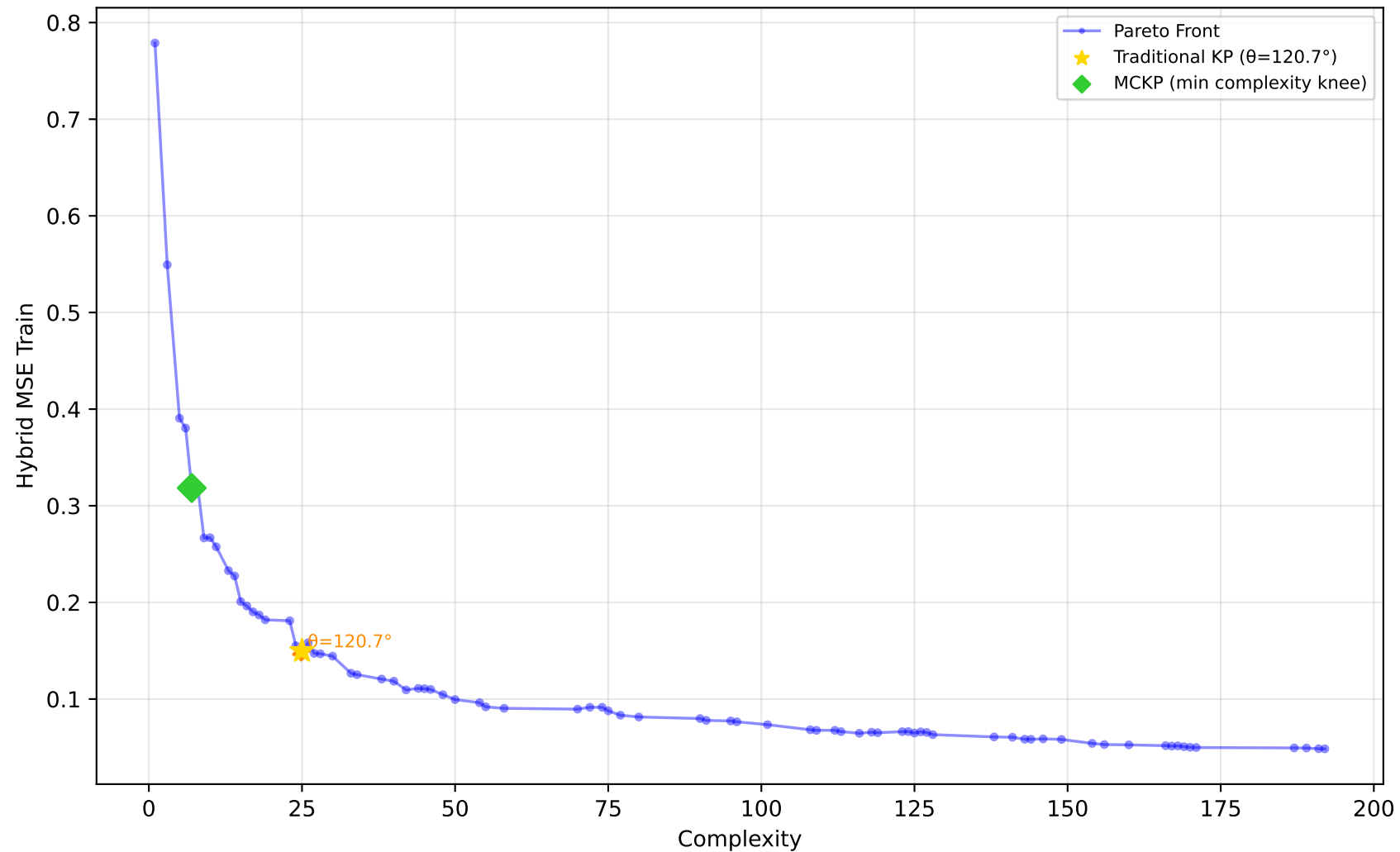
229_pwLinear - Run 13 - MVP - Hybrid MSE Train \lambda_1=0.50, \lambda_2=0.00, \lambda_3=0.00 | Difficulty: 1.00 | Method: hmr
