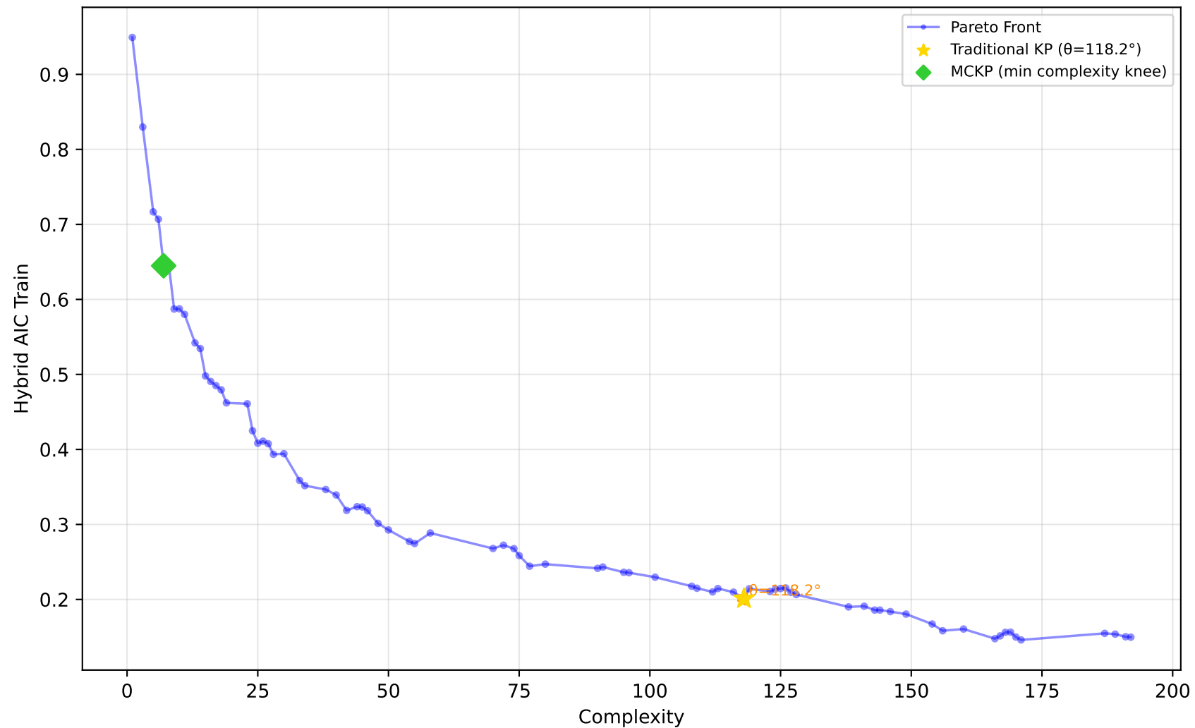
229_pwLinear - Run 13 - SVP - Hybrid AIC Train \lambda_1=0.50, \bar{\lambda}_2=0.10, \lambda_3=0.00 | Difficulty: 1.00 | Method: hmr
