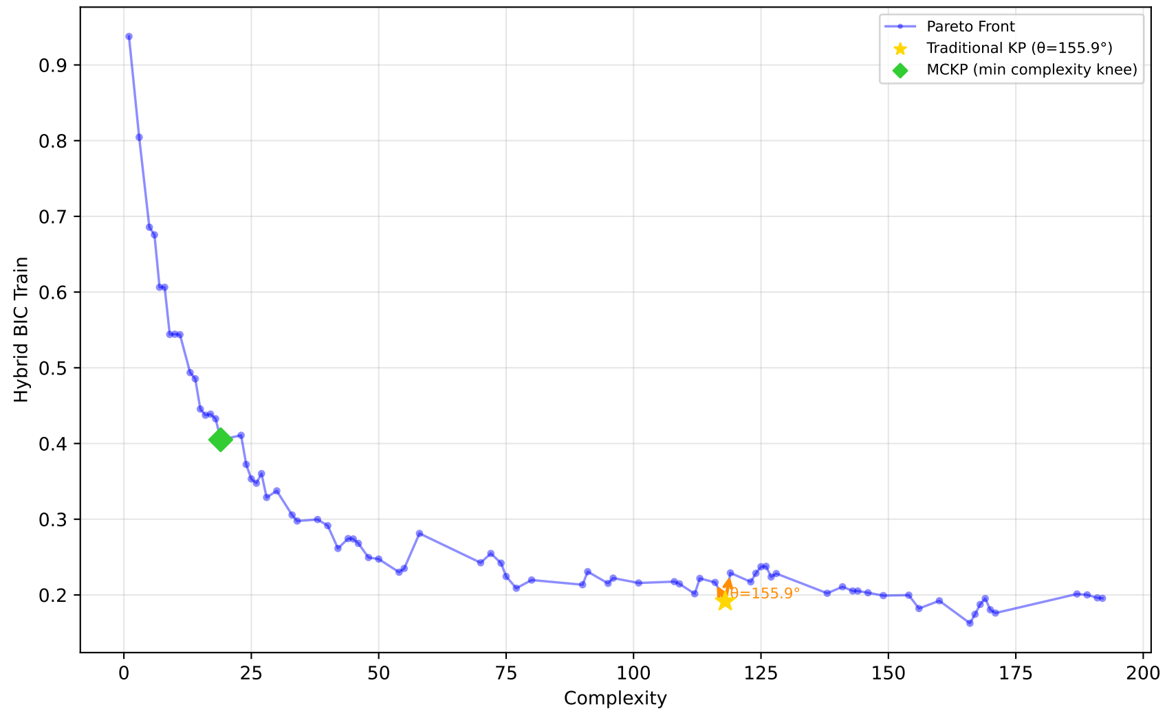
229_pwLinear - Run 13 - SVP - Hybrid BIC Train \lambda_1=0.50, \bar{\lambda}_2=0.00, \lambda_3=0.00 | Difficulty: 1.00 | Method: hmr
