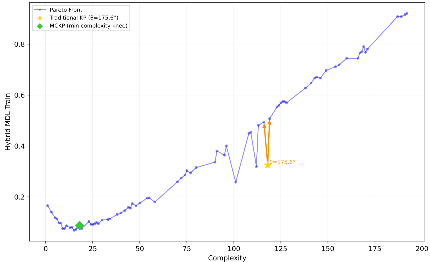
229_pwLinear - Run 13 - SVP - Hybrid MDL Train \lambda_1=0.50, \bar{\lambda}_2=0.10, \lambda_3=0.00 | Difficulty: 1.00 | Method: hmr
