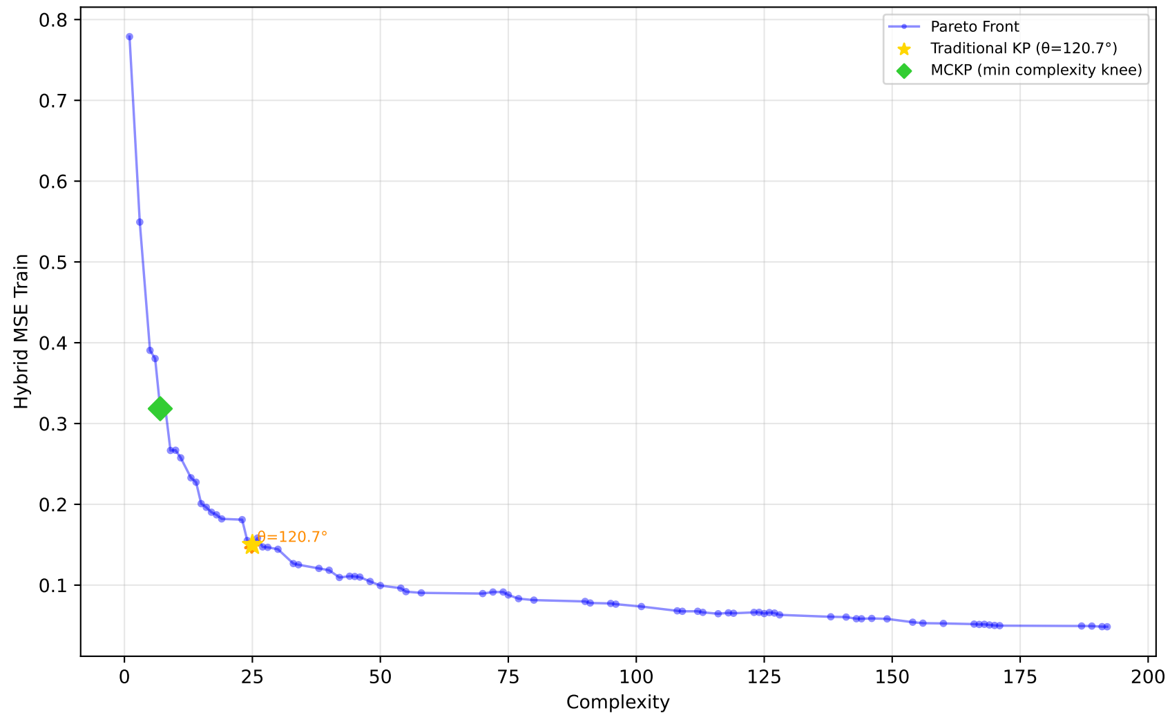
229_pwLinear - Run 13 - SVP - Hybrid MSE Train \lambda_1=0.50, \bar{\lambda}_2=0.00, \lambda_3=0.00 | Difficulty: 1.00 | Method: hmr
