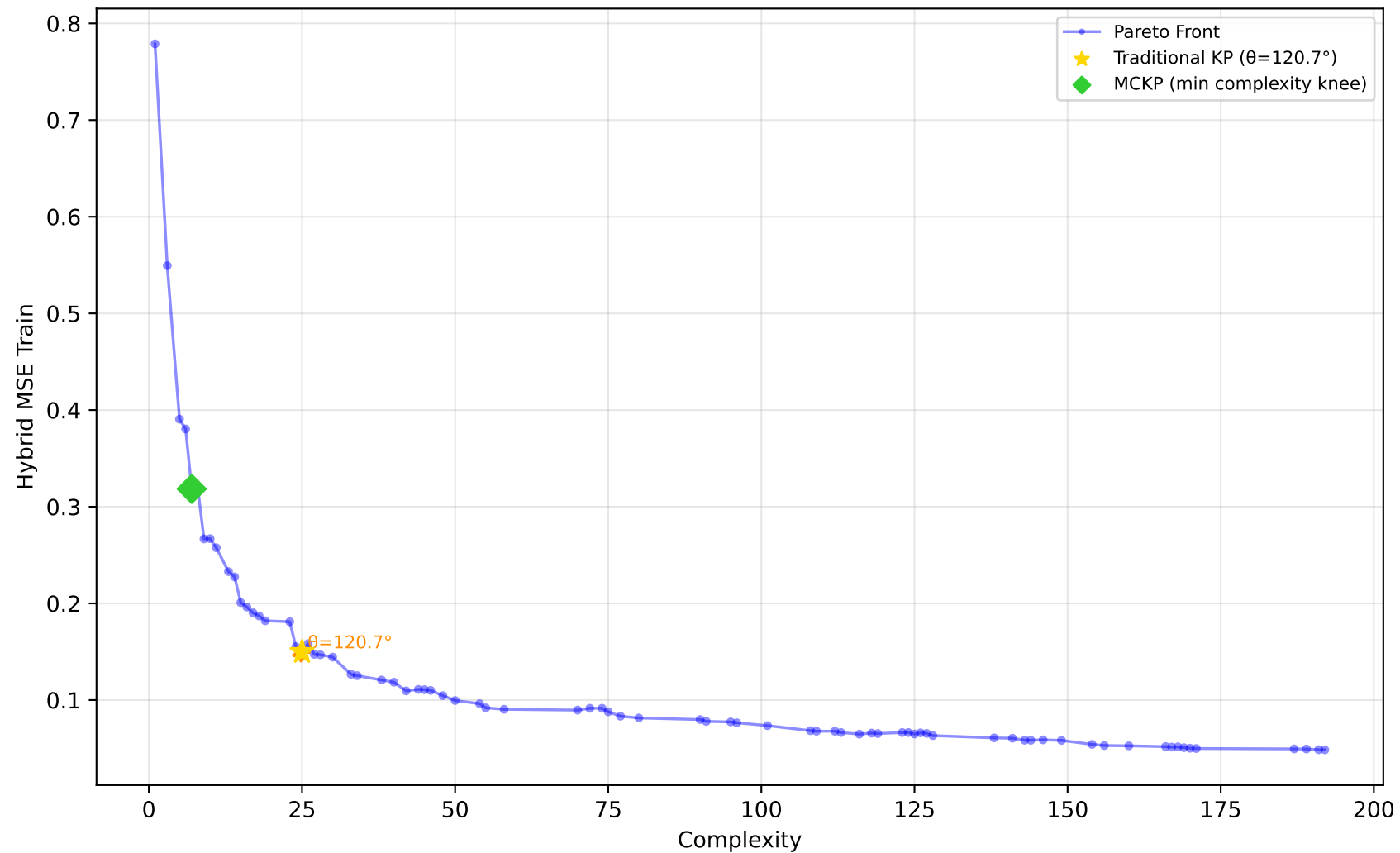
229_pwLinear - Run 13 - SVP - Hybrid MSE Train \lambda_1=0.50, \bar{\lambda}_2=0.10, \lambda_3=0.00 | Difficulty: 1.00 | Method: hmr
