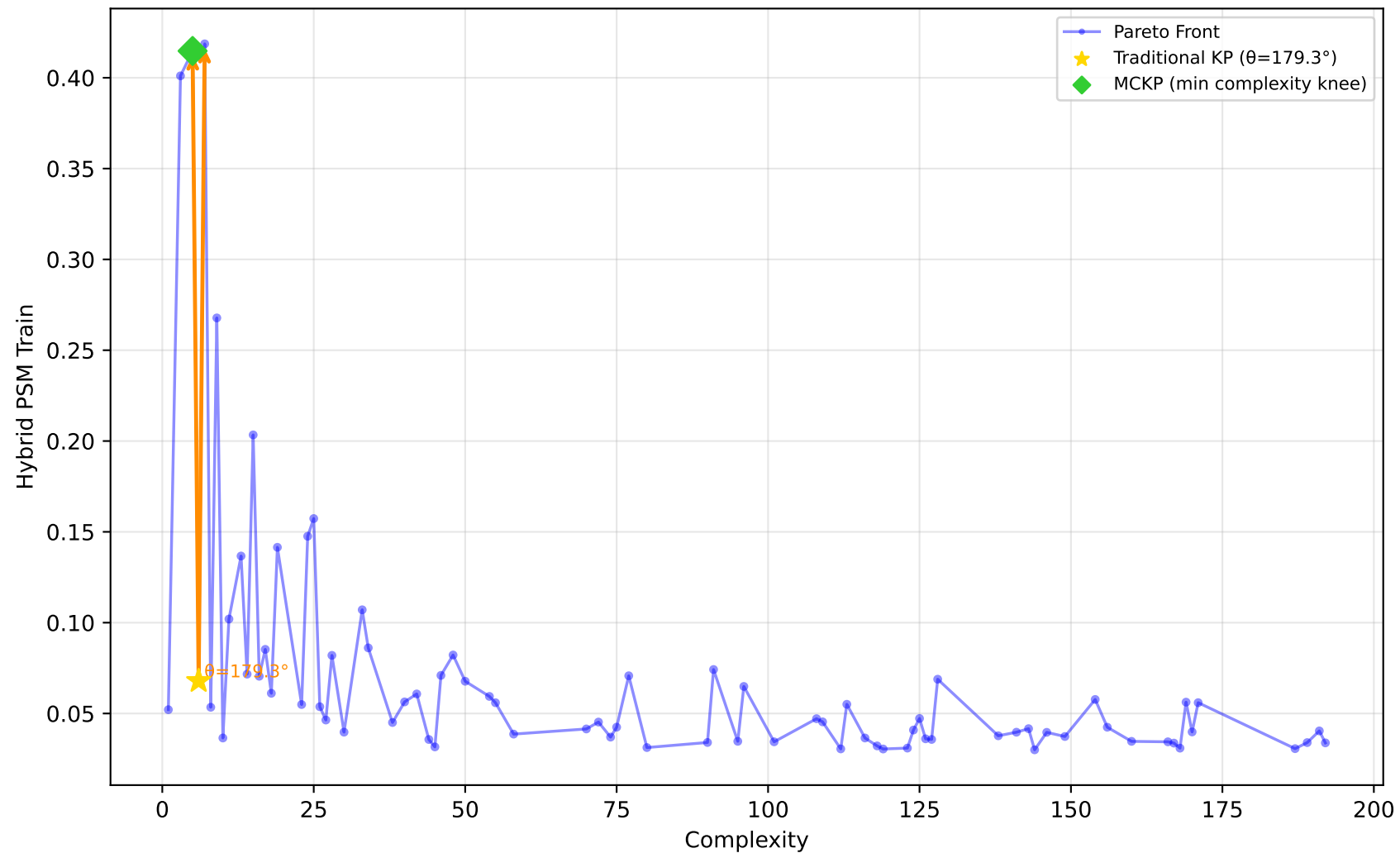
229_pwLinear - Run 13 - SVP - Hybrid PSM Train \lambda_1=0.50, \bar{\lambda}_2=0.00, \lambda_3=0.00 | Difficulty: 1.00 | Method: hmr
