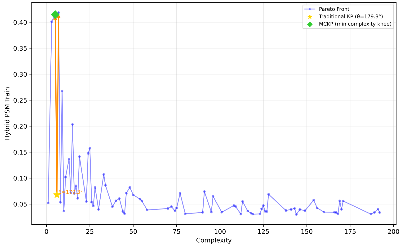
229_pwLinear - Run 13 - SVP - Hybrid PSM Train \lambda_1=0.50, \bar{\lambda}_2=0.10, \lambda_3=0.00 | Difficulty: 1.00 | Method: hmr
