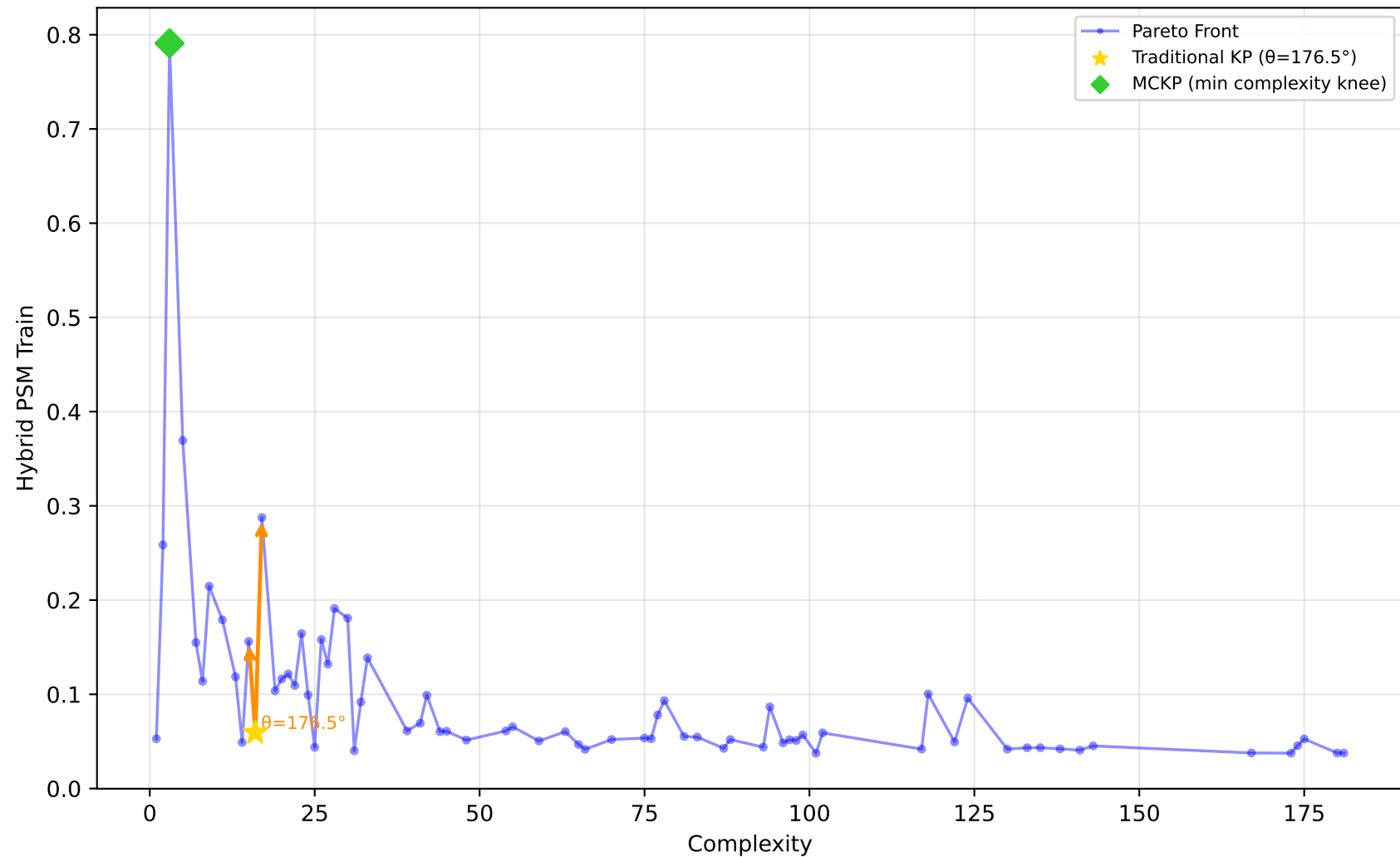
229_pwLinear - Run 14 - MVP - Hybrid PSM Train \lambda_1=0.50, \lambda_2=0.00, \lambda_3=0.00 | Difficulty: 1.00 | Method: hmr
