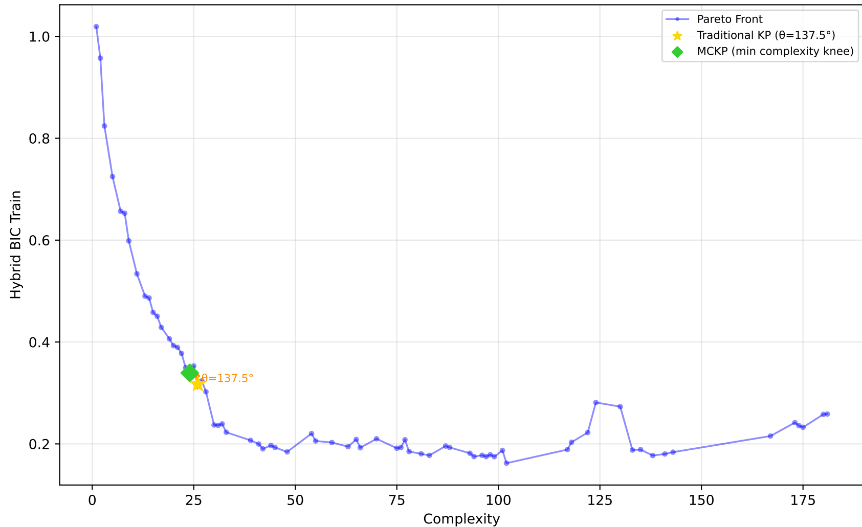
229_pwLinear - Run 14 - SVP - Hybrid BIC Train \lambda_1=0.50, \lambda_2=0.10, \lambda_3=0.00 | Difficulty: 1.00 | Method: hmr
