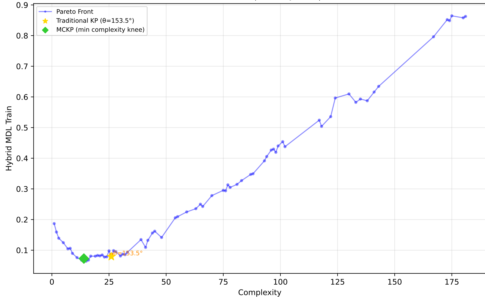
229_pwLinear - Run 14 - SVP - Hybrid MDL Train \lambda_1=0.50, \lambda_2=0.00, \lambda_3=0.00 | Difficulty: 1.00 | Method: hmr
