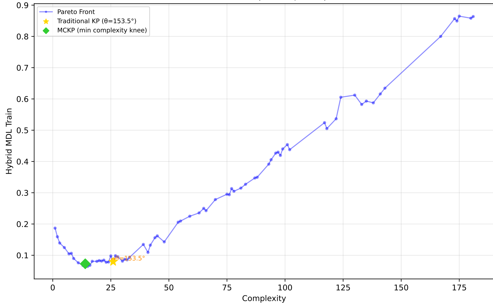
229_pwLinear - Run 14 - SVP - Hybrid MDL Train \lambda_1=0.50, \lambda_2=0.10, \lambda_3=0.00 | Difficulty: 1.00 | Method: hmr
