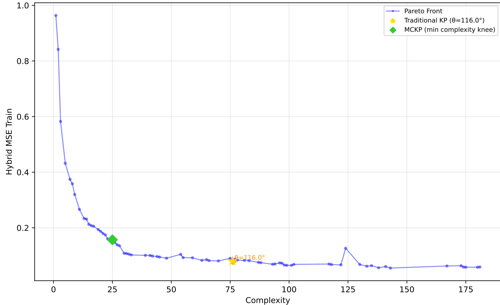
229_pwLinear - Run 14 - SVP - Hybrid MSE Train \lambda_1=0.50, \lambda_2=0.10, \lambda_3=0.00 | Difficulty: 1.00 | Method: hmr
