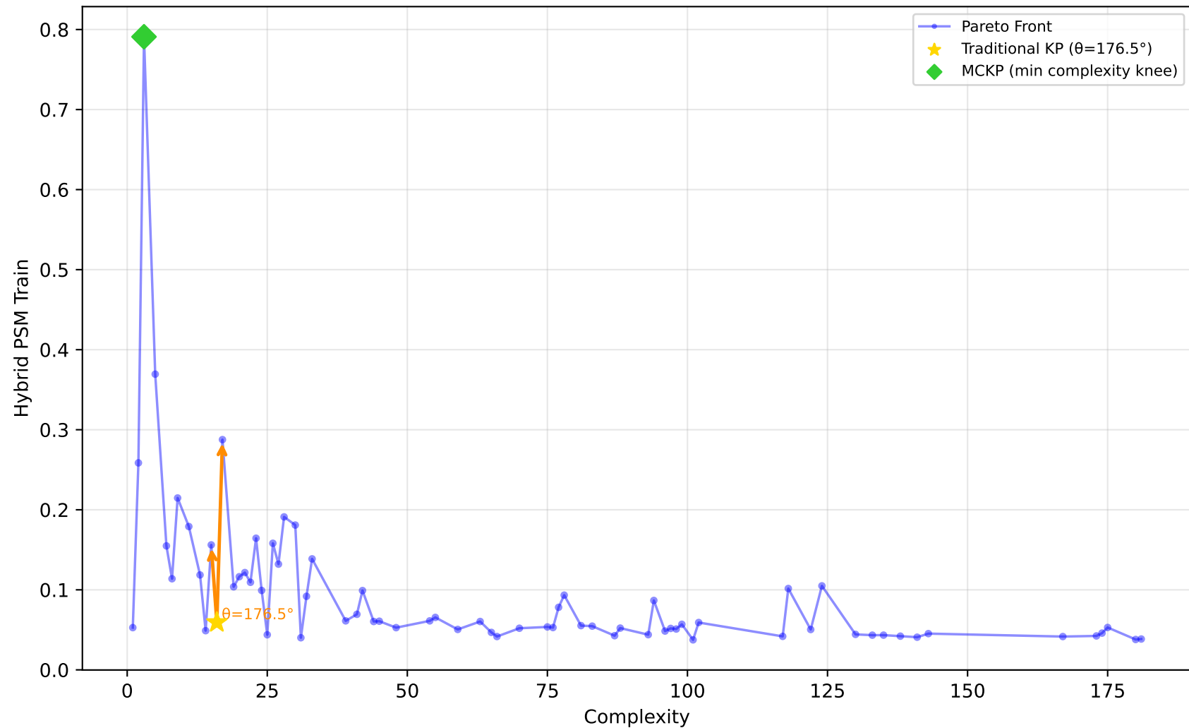
229_pwLinear - Run 14 - SVP - Hybrid PSM Train \lambda_1=0.50, \bar{\lambda}_2=0.10, \lambda_3=0.00 | Difficulty: 1.00 | Method: hmr
