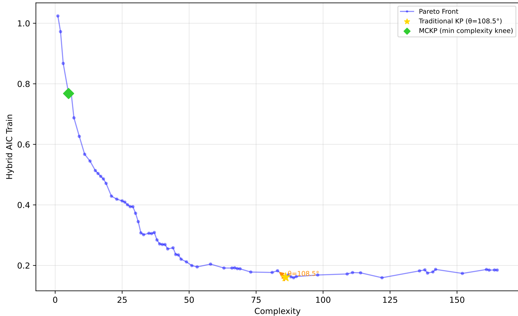
229_pwLinear - Run 15 - MVP - Hybrid AIC Train \lambda_1=0.50, \bar{\lambda}_2=0.00, \lambda_3=0.00 | Difficulty: 1.00 | Method: hmr
