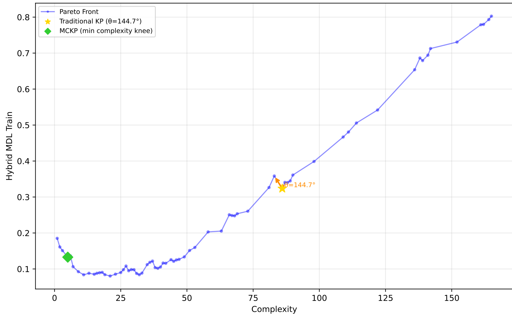
229_pwLinear - Run 15 - MVP - Hybrid MDL Train \lambda_1=0.50, \lambda_2=0.00, \lambda_3=0.00 | Difficulty: 1.00 | Method: hmr
