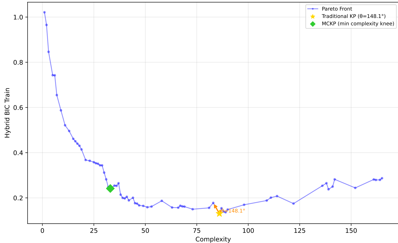
229_pwLinear - Run 15 - SVP - Hybrid BIC Train \lambda_1=0.50, \lambda_2=0.00, \lambda_3=0.00 | Difficulty: 1.00 | Method: hmr
