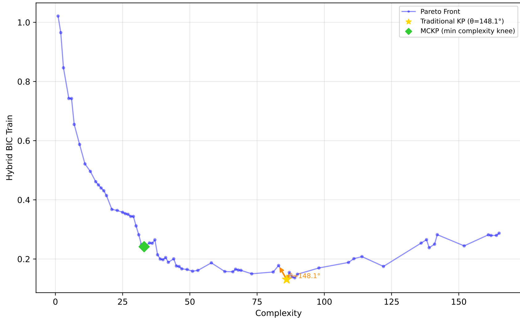
229_pwLinear - Run 15 - SVP - Hybrid BIC Train \lambda_1=0.50, \lambda_2=0.10, \lambda_3=0.00 | Difficulty: 1.00 | Method: hmr
