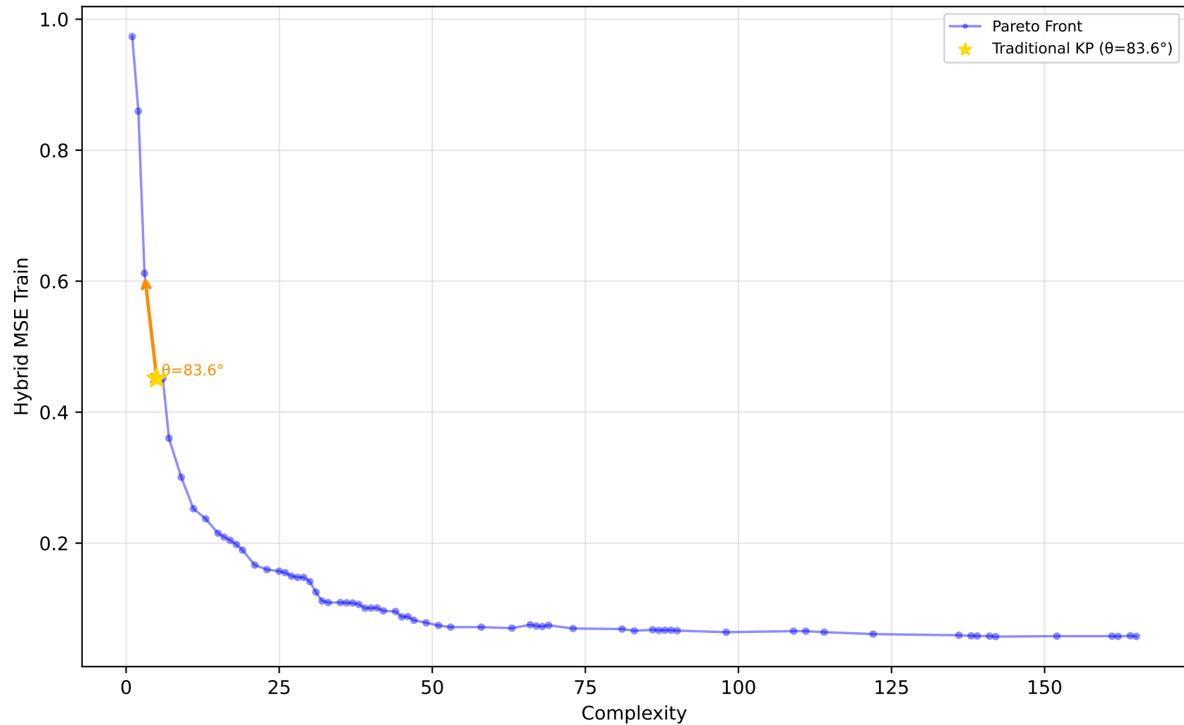
229_pwLinear - Run 15 - SVP - Hybrid MSE Train \lambda_1=0.50, \lambda_2=0.00, \lambda_3=0.00 | Difficulty: 1.00 | Method: hmr
