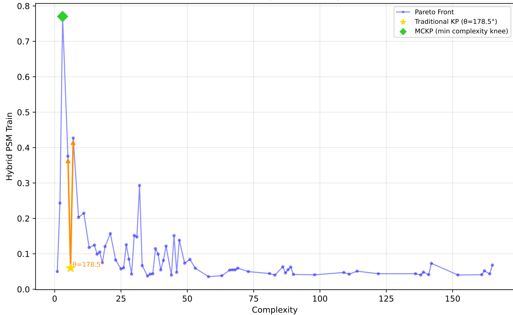
229_pwLinear - Run 15 - SVP - Hybrid PSM Train \lambda_1=0.50, \bar{\lambda}_2=0.10, \lambda_3=0.00 | Difficulty: 1.00 | Method: hmr
