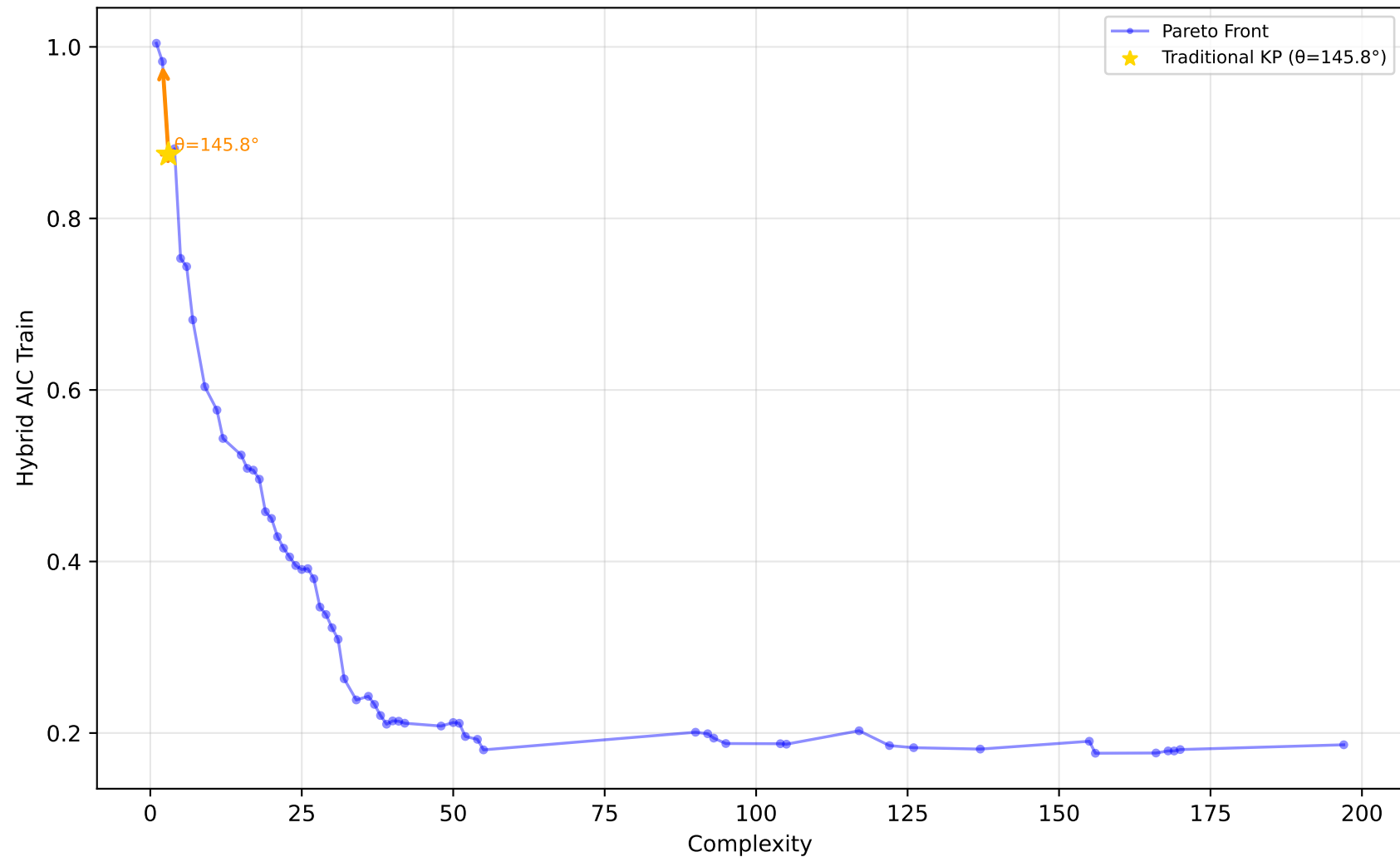
229_pwLinear - Run 16 - MVP - Hybrid AIC Train \lambda_1=0.50, \lambda_2=0.00, \lambda_3=0.00 | Difficulty: 1.00 | Method: hmr
