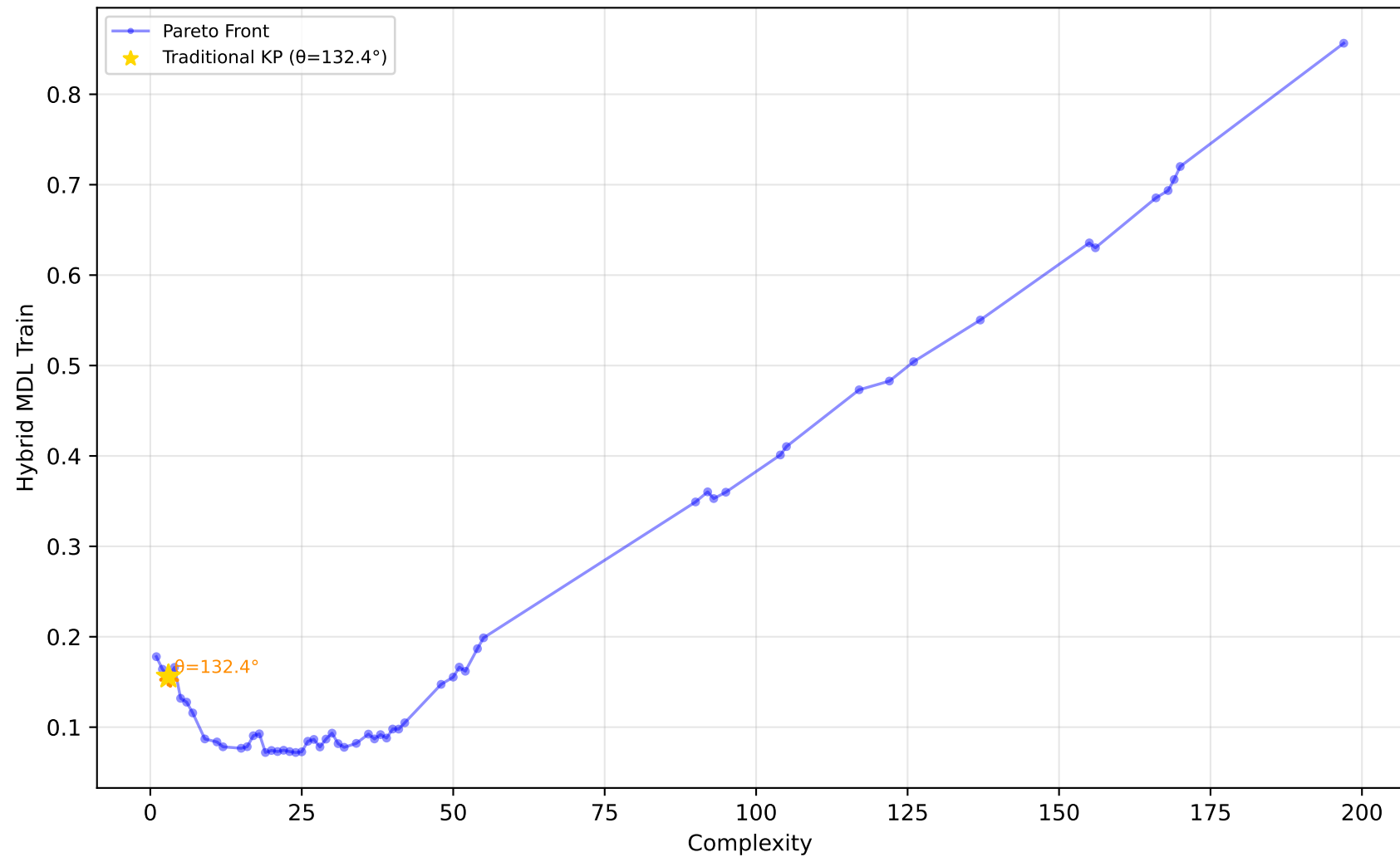
229_pwLinear - Run 16 - MVP - Hybrid MDL Train \lambda_1=0.50, \lambda_2=0.00, \lambda_3=0.00 | Difficulty: 1.00 | Method: hmr
