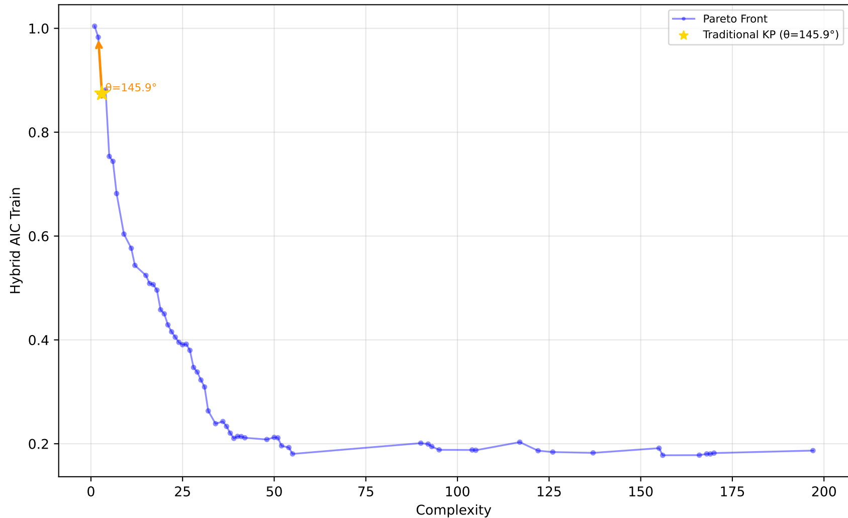
229_pwLinear - Run 16 - SVP - Hybrid AIC Train \lambda_1=0.50, \lambda_2=0.10, \lambda_3=0.00 | Difficulty: 1.00 | Method: hmr
