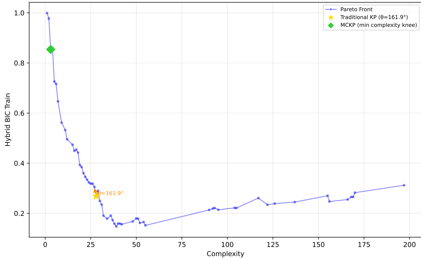
229_pwLinear - Run 16 - SVP - Hybrid BIC Train \lambda_1=0.50, \bar{\lambda}_2=0.00, \lambda_3=0.00 | Difficulty: 1.00 | Method: hmr
