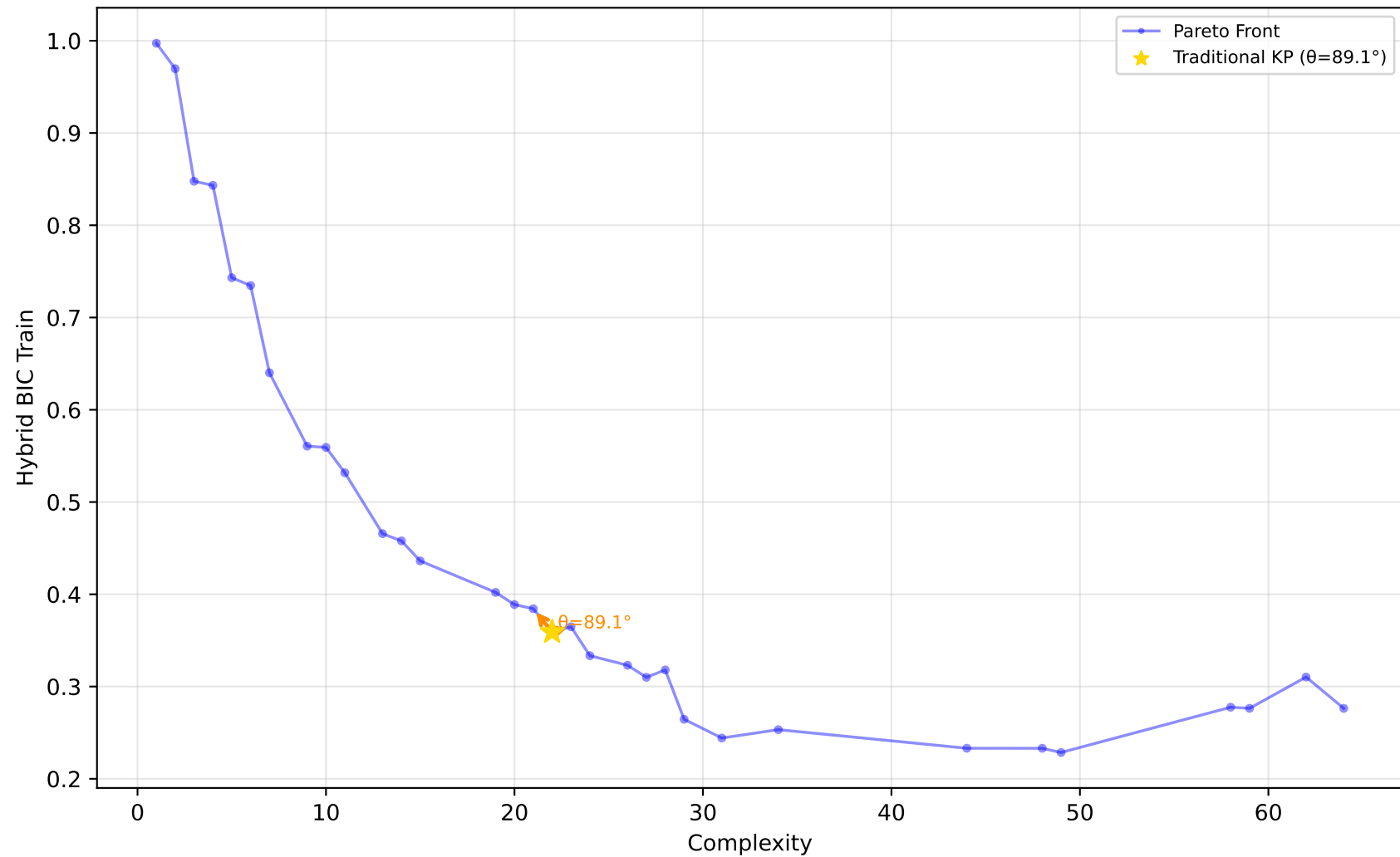
229_pwLinear - Run 17 - MVP - Hybrid BIC Train \lambda_1=0.50, \bar{\lambda}_2=0.00, \lambda_3=0.00 | Difficulty: 1.00 | Method: hmr
