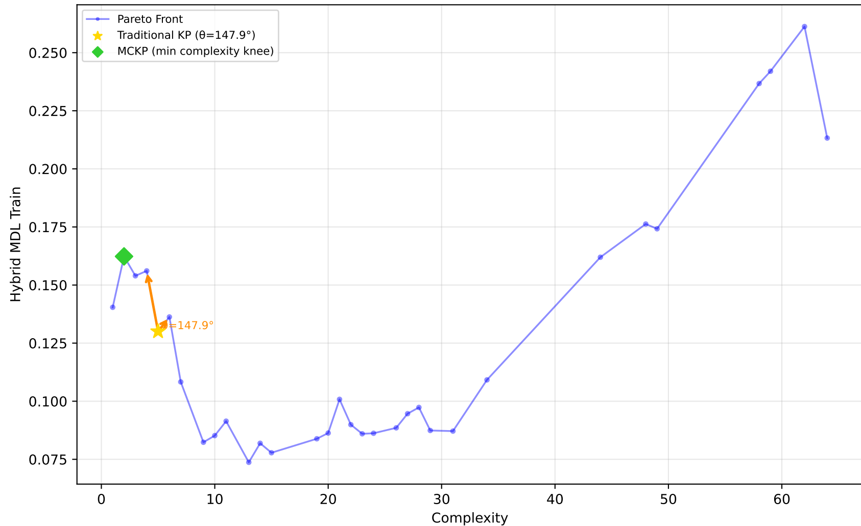
229_pwLinear - Run 17 - MVP - Hybrid MDL Train \lambda_1=0.50, \lambda_2=0.00, \lambda_3=0.00 | Difficulty: 1.00 | Method: hmr
