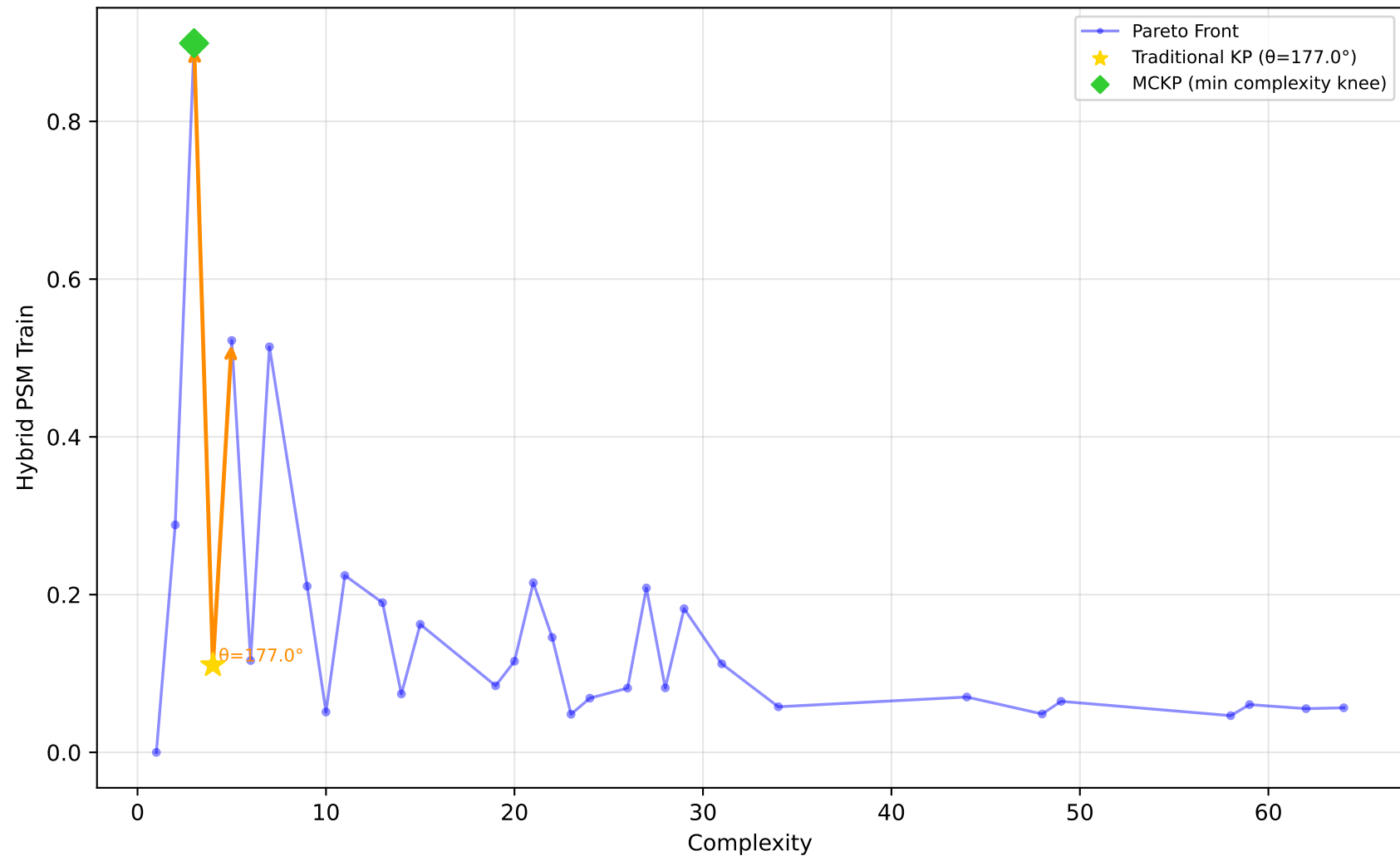
229_pwLinear - Run 17 - MVP - Hybrid PSM Train \lambda_1=0.50, \lambda_2=0.00, \lambda_3=0.00 | Difficulty: 1.00 | Method: hmr
