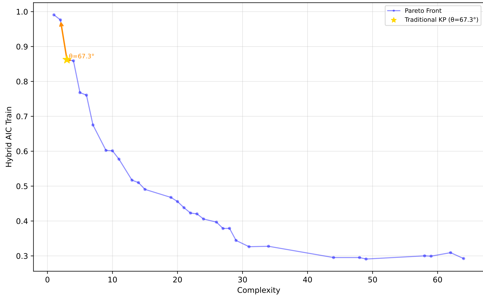
229_pwLinear - Run 17 - SVP - Hybrid AIC Train \lambda_1=0.50, \lambda_2=0.10, \lambda_3=0.00 | Difficulty: 1.00 | Method: hmr
