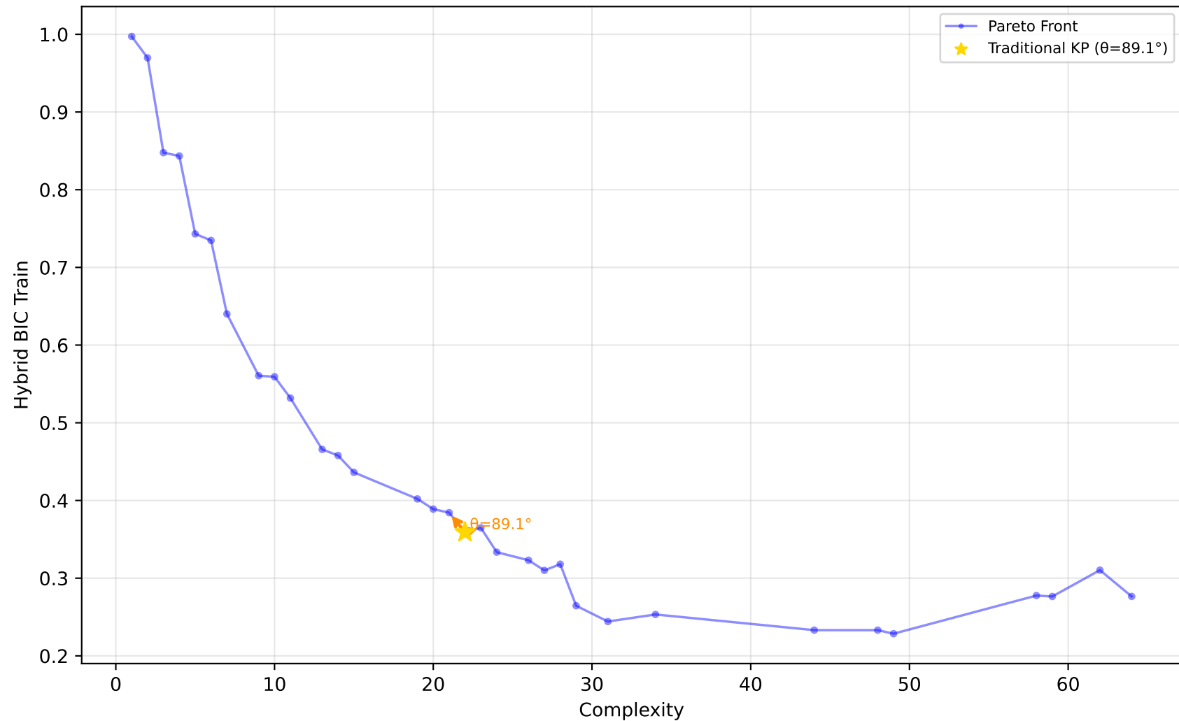
229_pwLinear - Run 17 - SVP - Hybrid BIC Train \lambda_1=0.50, \lambda_2=0.10, \lambda_3=0.00 | Difficulty: 1.00 | Method: hmr
