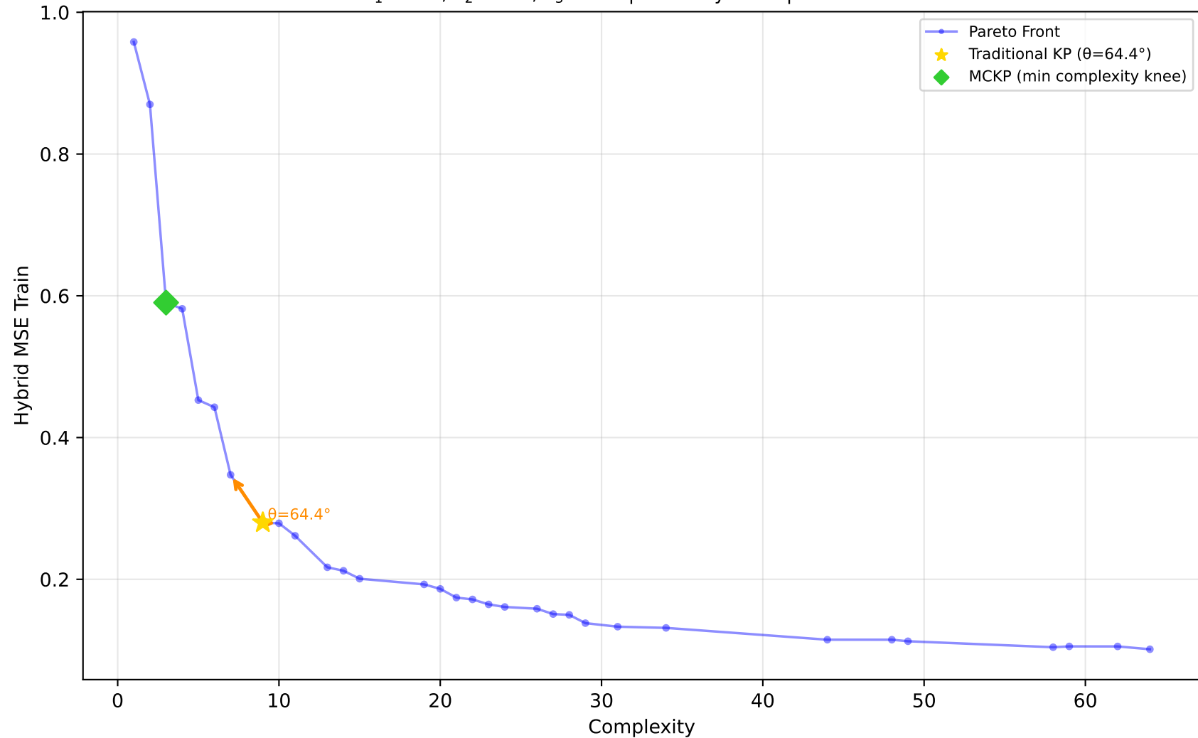
229_pwLinear - Run 17 - SVP - Hybrid MSE Train \lambda_1=0.50, \bar{\lambda}_2=0.00, \lambda_3=0.00 | Difficulty: 1.00 | Method: hmr
