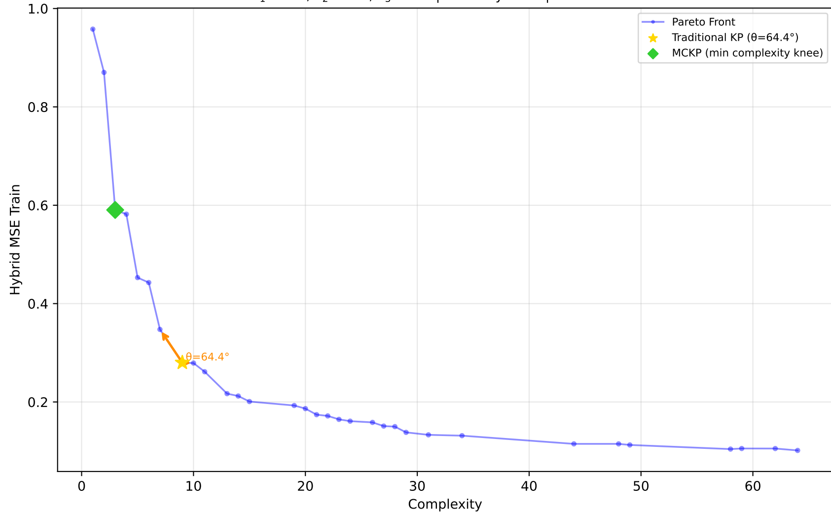
229_pwLinear - Run 17 - SVP - Hybrid MSE Train \lambda_1=0.50, \bar{\lambda}_2=0.10, \lambda_3=0.00 | Difficulty: 1.00 | Method: hmr
